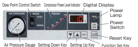
Control Panel
