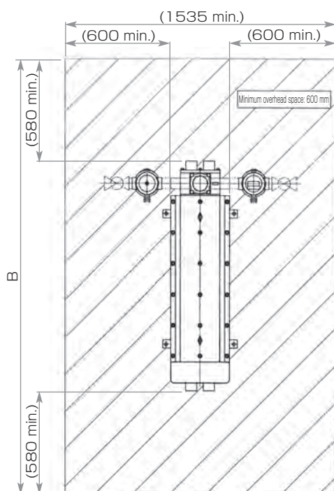
Installation and Maintenance Space
