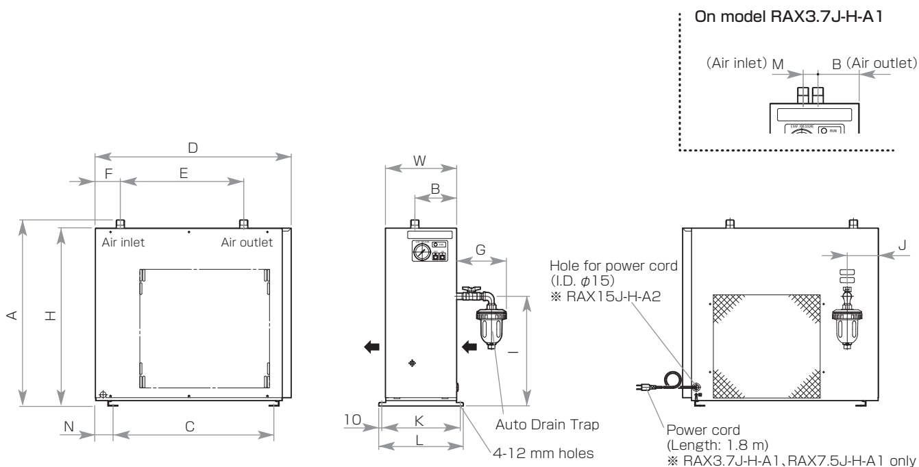
External Dimensions (Units:mm)
