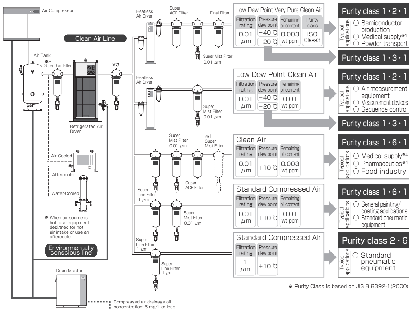
ISO 8573-1(1991)/JIS B 8392-1(2000) Contaminants and Purity Classes
