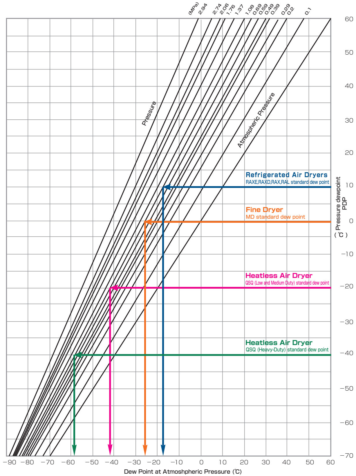
Dew Point Conversion Chart
