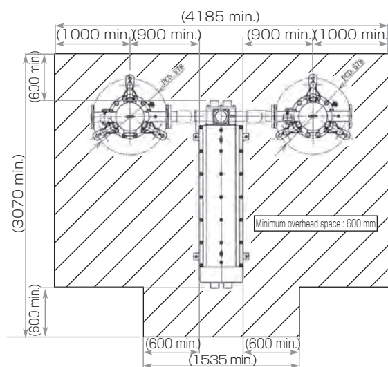
Installation and Maintenance Space
