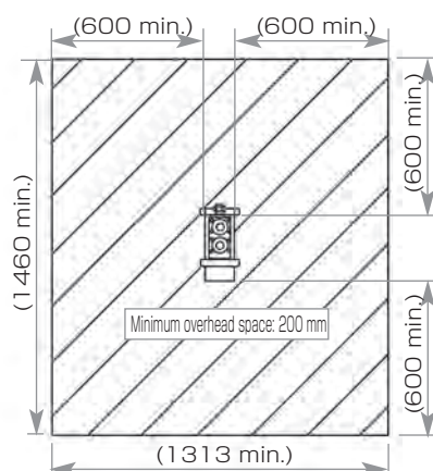
Installation and Maintenance Space
