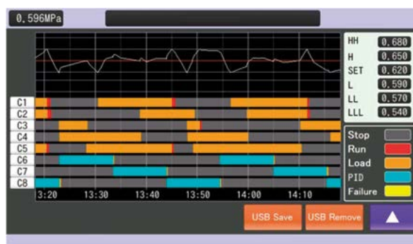
Graphic Display of operation status
