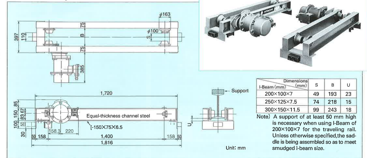
Dimensional diagram
