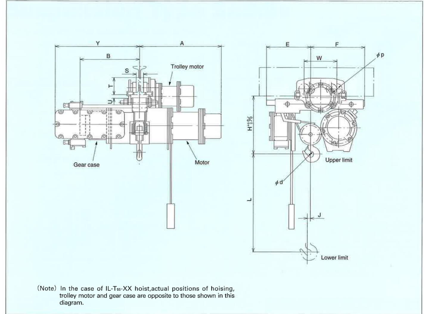
Dimensional diagram
