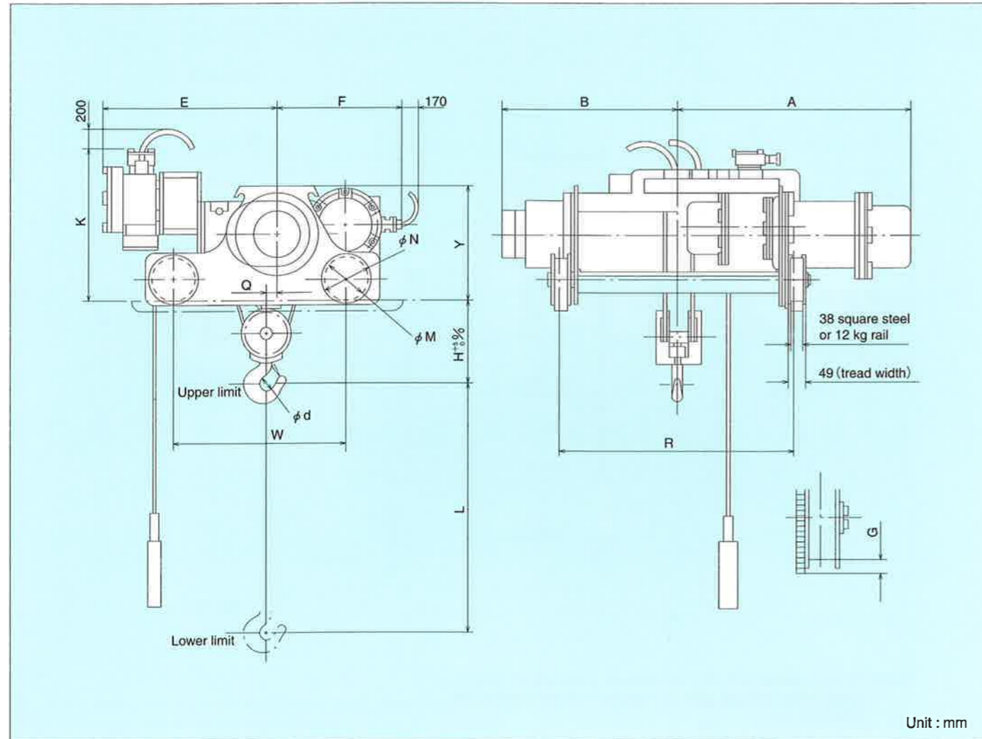
Dimensional diagram
