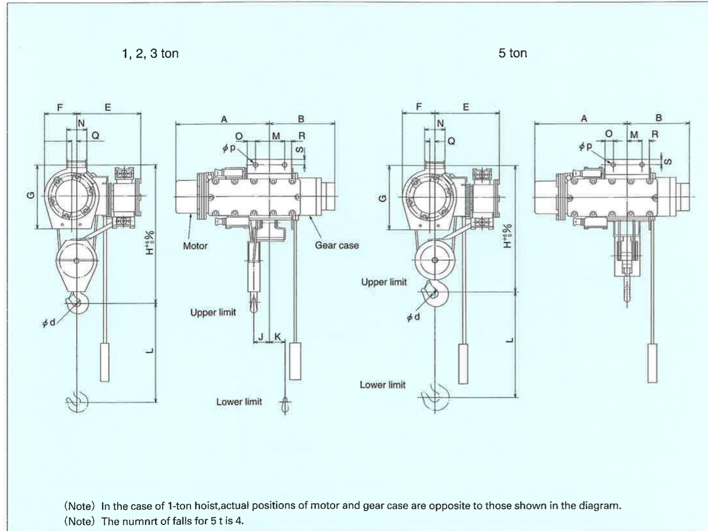
Dimensional diagram
