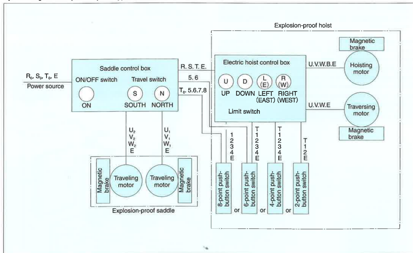
System diagram of explosion-proof type hoist crane
